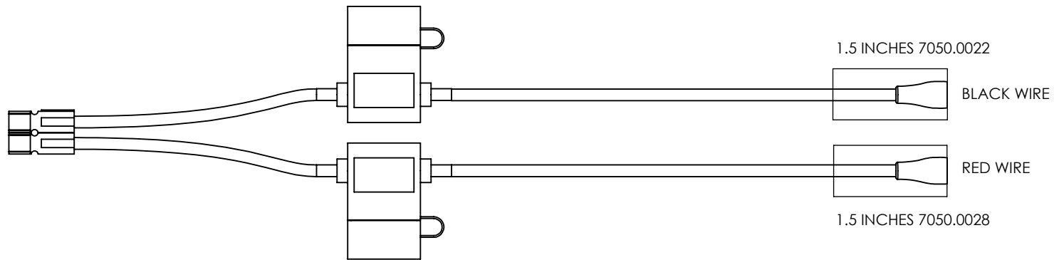
2435.0020 FUSE HOLDERS (INCLUDES FUSES, WIRES, AND CONNECTORS)
